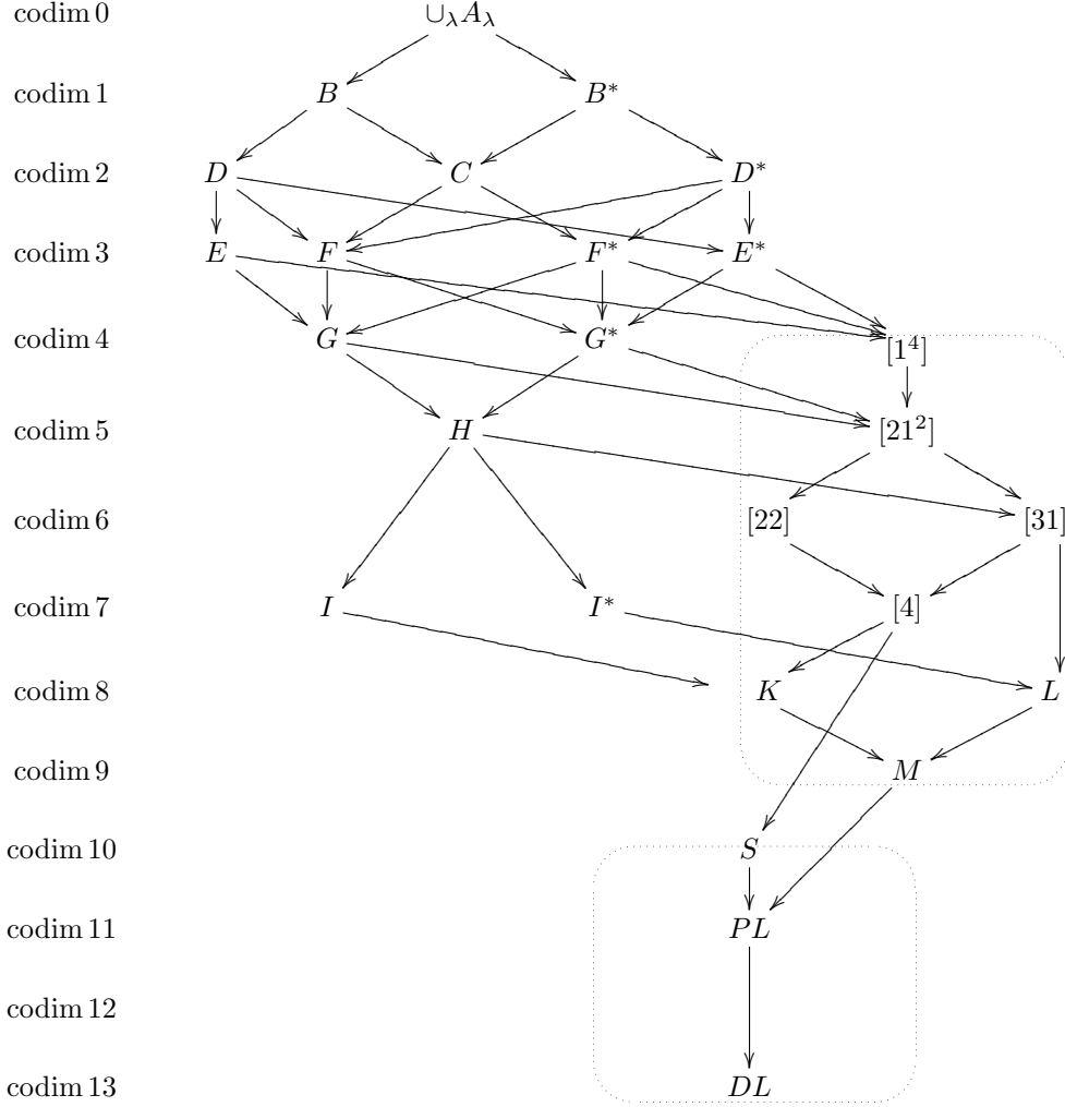
FIGURE 2. The hierarchy of Noc orbits
