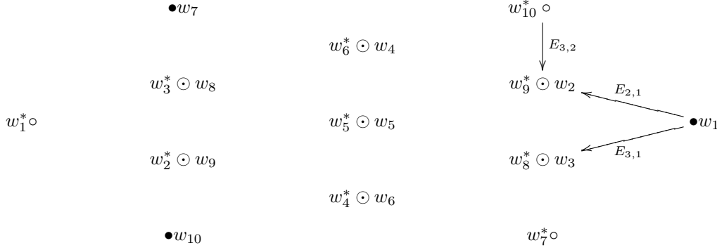
FIGURE 1. The 20 weights of \mathbf{P1}
